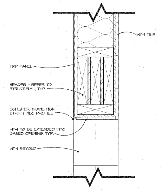
11 A-5.3 OUTSIDE CORNER DETAIL SCALE 6" = 1'-0"
