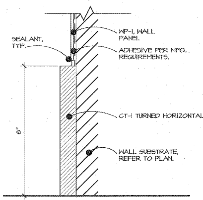
4 A-5.3 BASE DETAIL SCALE 6" = 1'-0"
