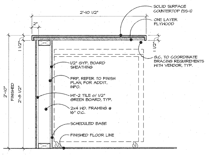
10 A-5.3 PARTIAL HT. WALL DETAIL SCALE 1 1/2" = 1'-0"
