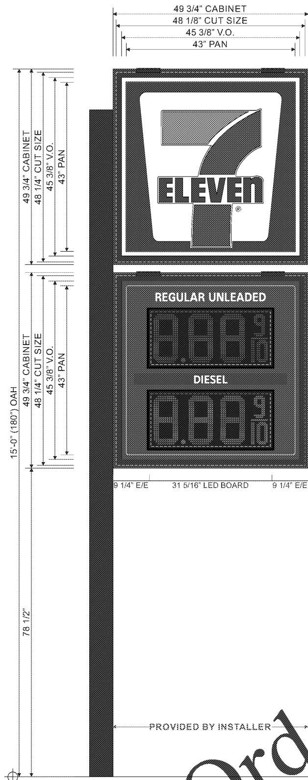
Face & Side Detail - M16 Main-ID & L162D D/F Diesel Signs - Pylon Sign Structure - Sign A 1/2" = 1'-0"
