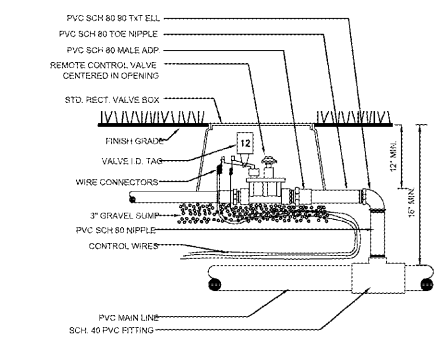
1 REMOTE CONTROL VALVE SCALE: NTS
