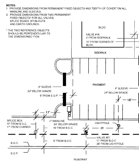
12 "AS BUILT" TYPICAL SCALE: NTS
