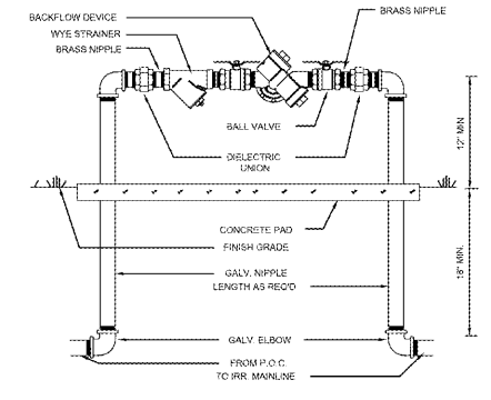
3 BACKFLOW PREVENTION DEVICE SCALE: NTS
