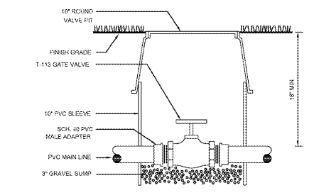
2 ISOLATION GATE VALVE SCALE: NTS
