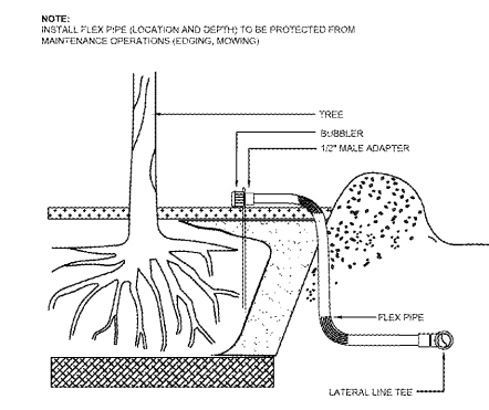
6 TREE BUBBLER SCALE: NTS
