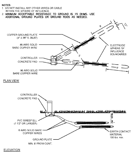
11 CONTROLLER GROUNDING SCALE: NTS
