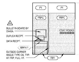
12 ASSOCIATES' ROOM ELEV. A1.2 14" x 14"
