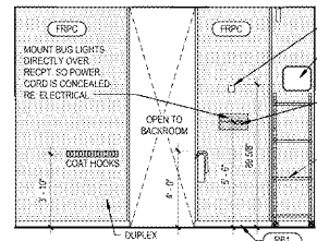
18 BACKROOM ELEV. A1.2 14" x 14"
