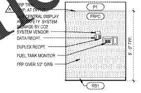
6 OFFICE ELEVATION A1.2 14" x 14"
