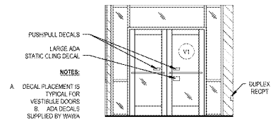
5 ADA DECAL DTL @ VESTIBULE DOOR A1.1 14" x 14"
