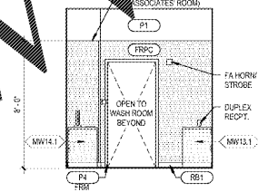
13 ASSOCIATES' ROOM ELEV. A1.2 14" x 14"
