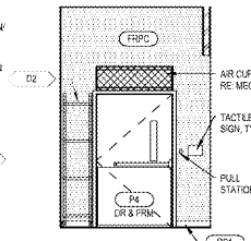
17 BACKROOM ELEV. A1.2 14" x 14"
