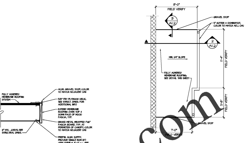
CANOPY DETAIL 5 SCALE: 1 1/2" = 1'-0"
