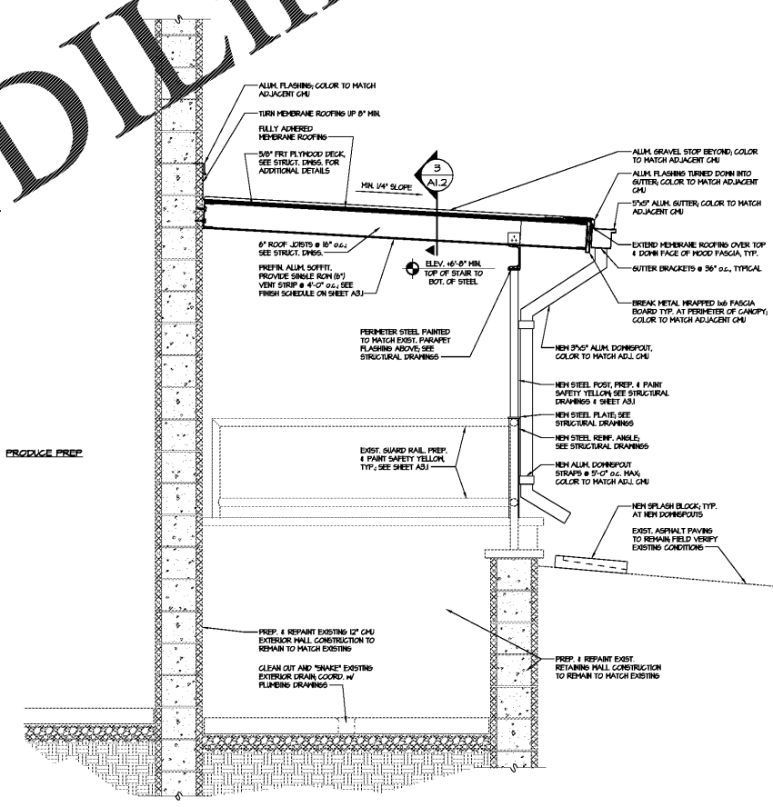
SECTION AT NEW EXTERIOR CANOPY 2 SCALE: 3/4" = 1'-0"
