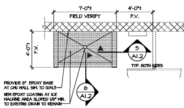
PLAN AT ICE MACHINE 4 SCALE: 1/4" = 1'-0"
