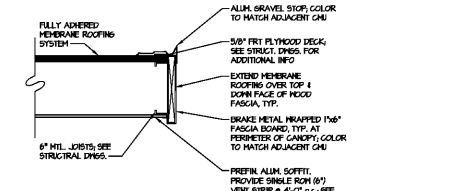
CANOPY DETAIL 5 SCALE: 1 1/2" = 1'-0"
