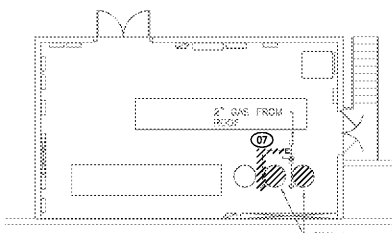
MEZZANINE PLAN-GAS
