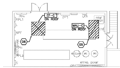
HVAC DEMOLITION MEZZANINE PLAN
