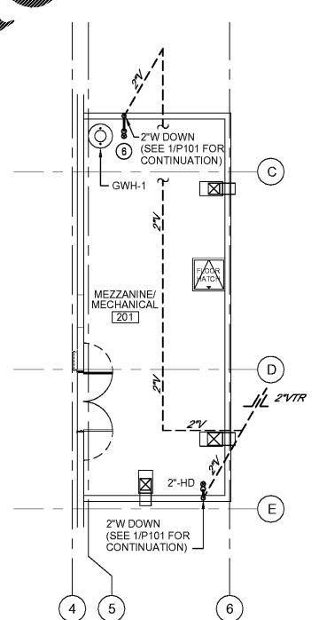
② MEZZANINE WASTE PIPING PLAN SCALE: 1/8" = 1'-0"
